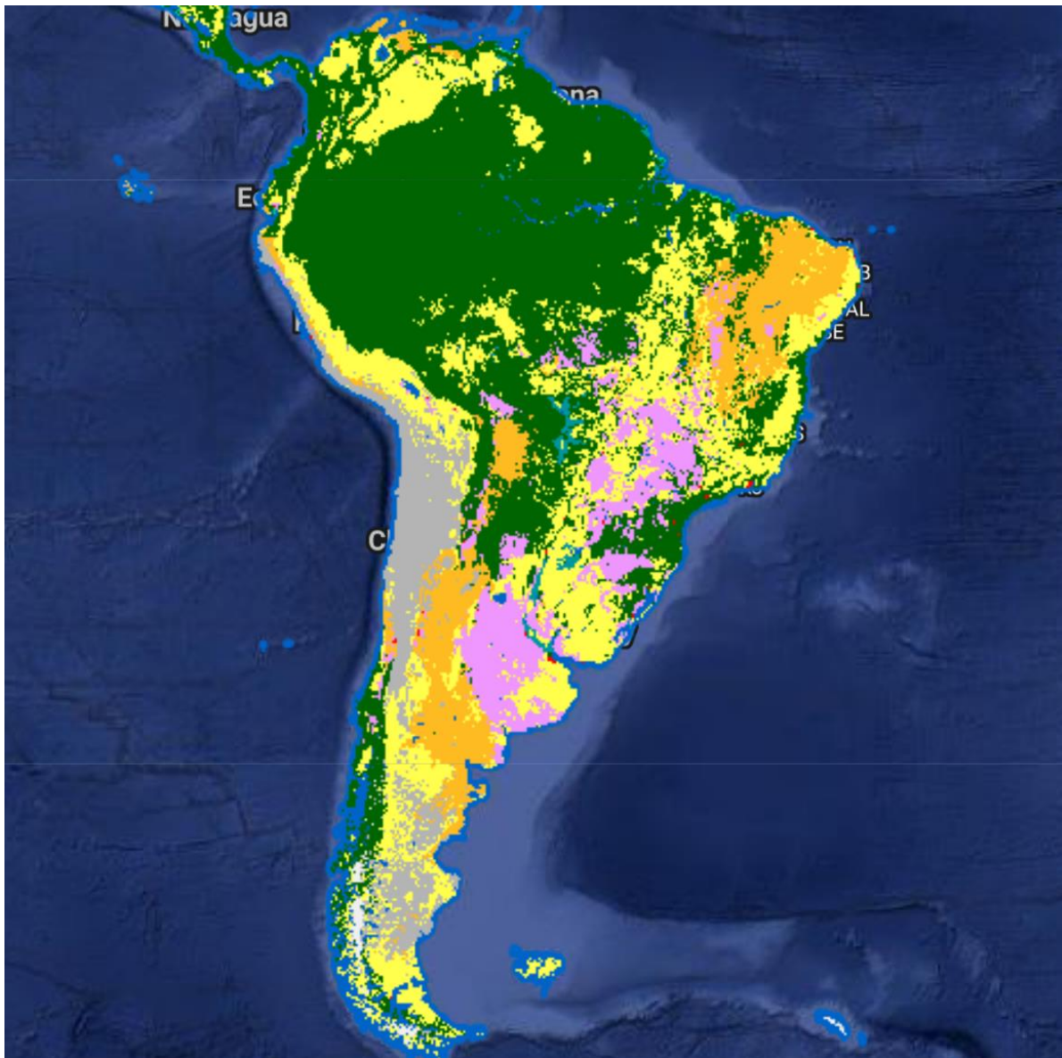
Figura 7 WorldCover 10 m 2020 – Sud America
